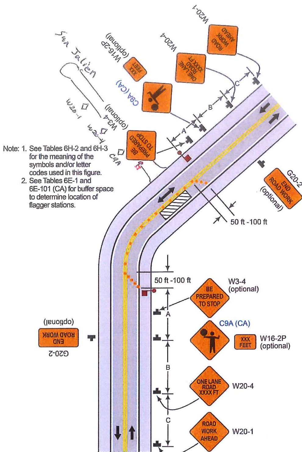
Typical Application 10
